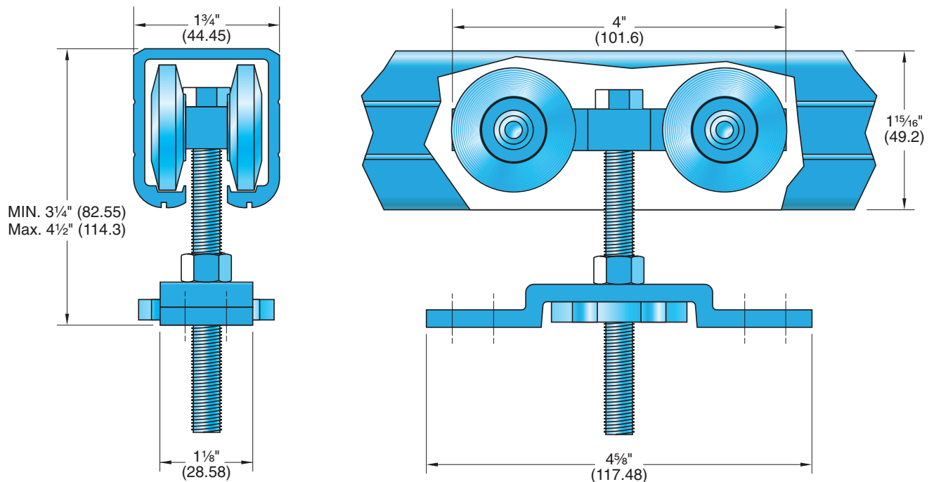
C-995 Hanger with C-204 Track Detail
