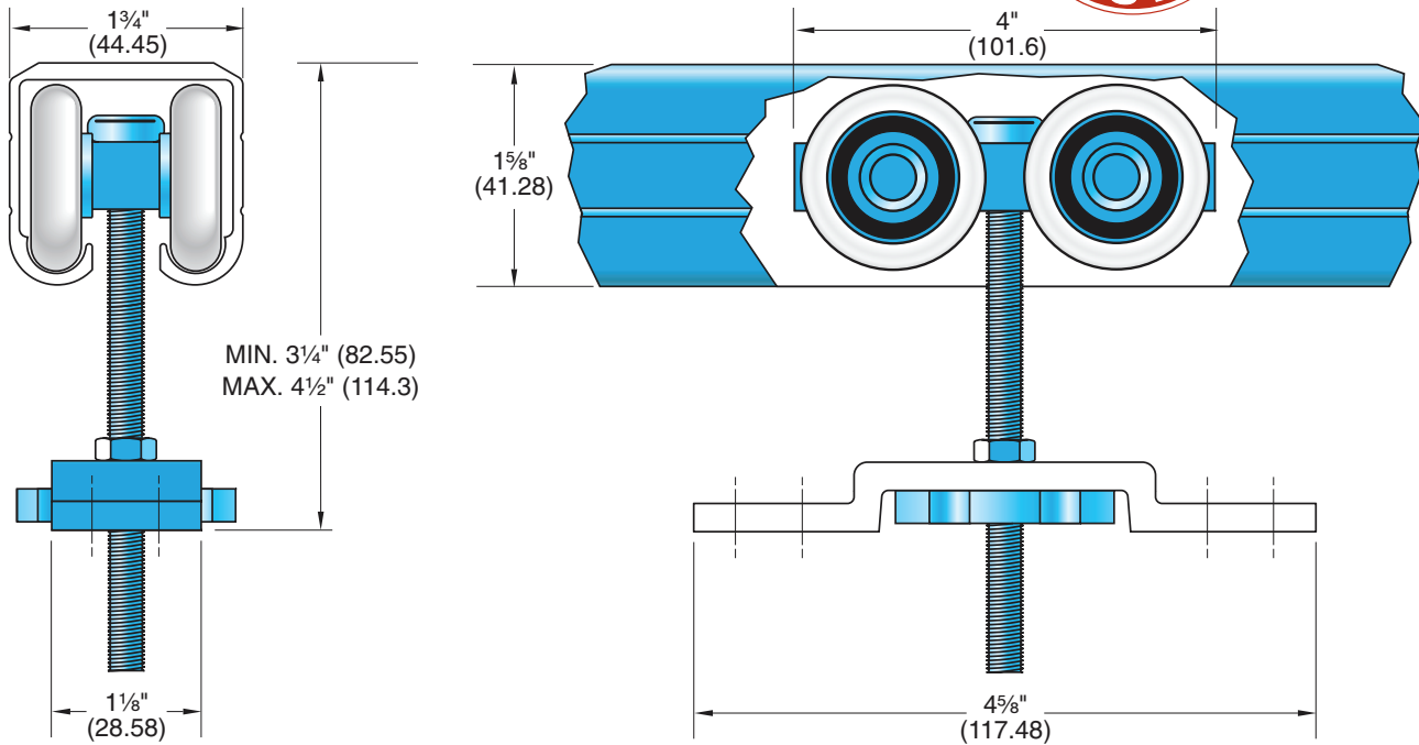
C-994 Hanger with C-104 Track Detail Curved track available
