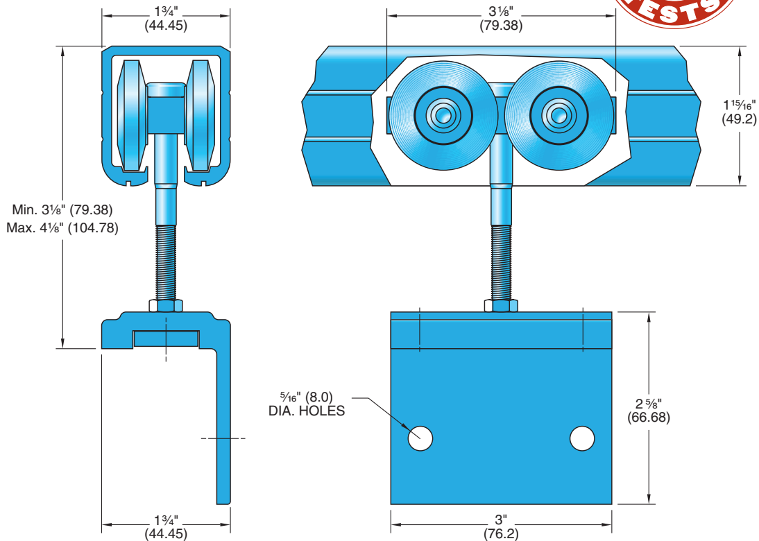
C-203-4 Hanger with C-204 Track Detail
