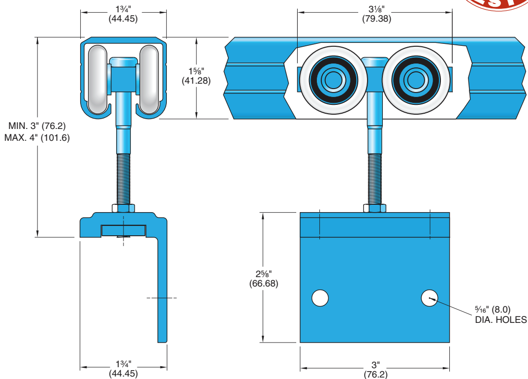
C-103-4 Hanger with C-104 track detail curved track available
