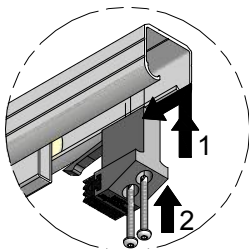
(CDC-911 IS SHOWN WITH C-104 TRACK AND C-911 HANGER)
