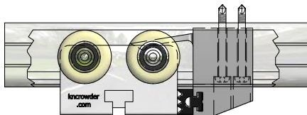
(CDC-911 IS SHOWN WITH C-104 TRACK AND C-911 HANGER)
