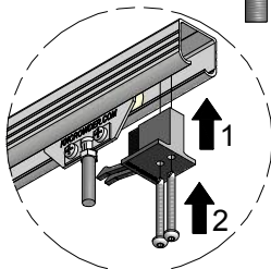
(CDC-400 IS SHOWN WITH C-400 SERIES TRACK AND HANGER)
